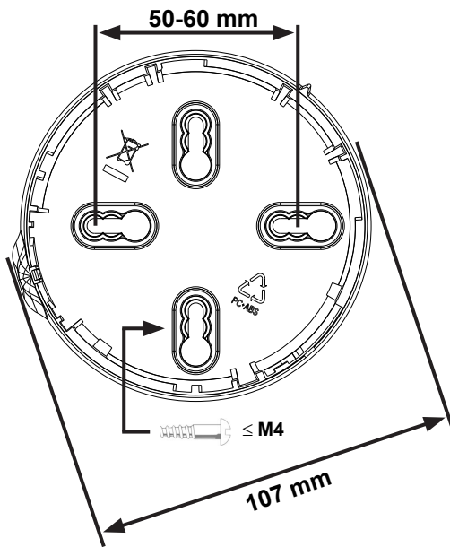
Figure 1: B501RF Mounting
