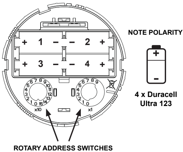
Figure 4: Battery Installation and Rotary Address Switches
