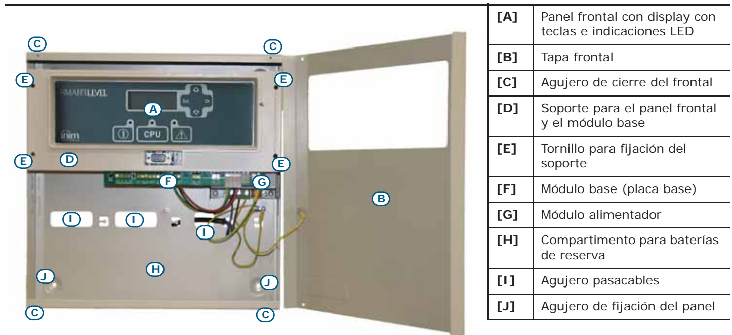
Figura 6 - Interior de SPS24060G
