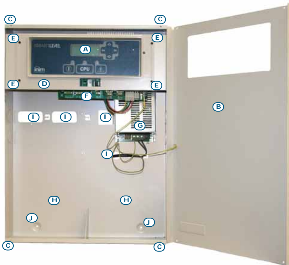
Figura 7 - Interior de SPS24160G
