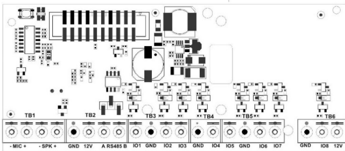
Figure 2.2 – Location of pinouts
