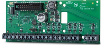
Fig. 1 Modulo Expander ioXpander-8
