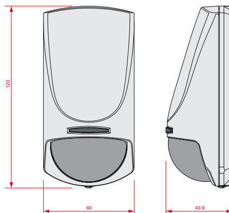
Air2-XDTP200W, Air2-XIRP200W - dimensiones
