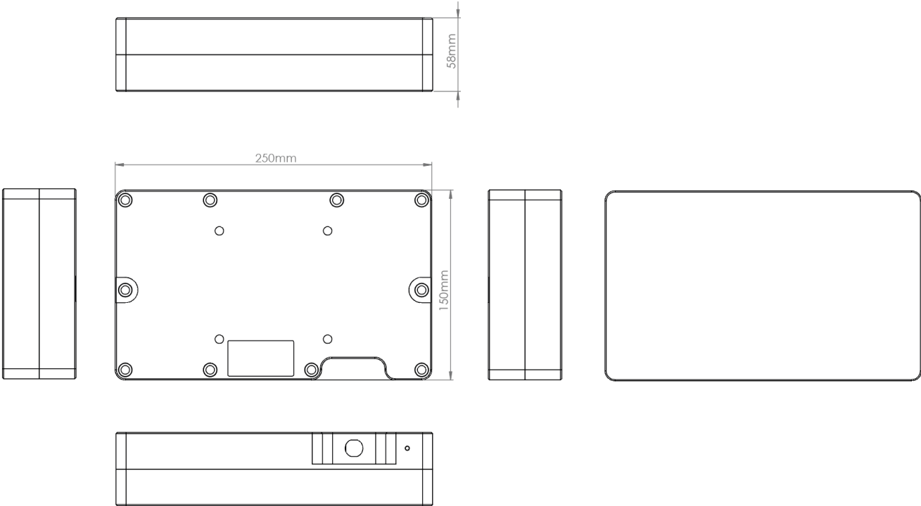
Figure 1: SR 150, 250 & 500 radar sensor outline drawing
