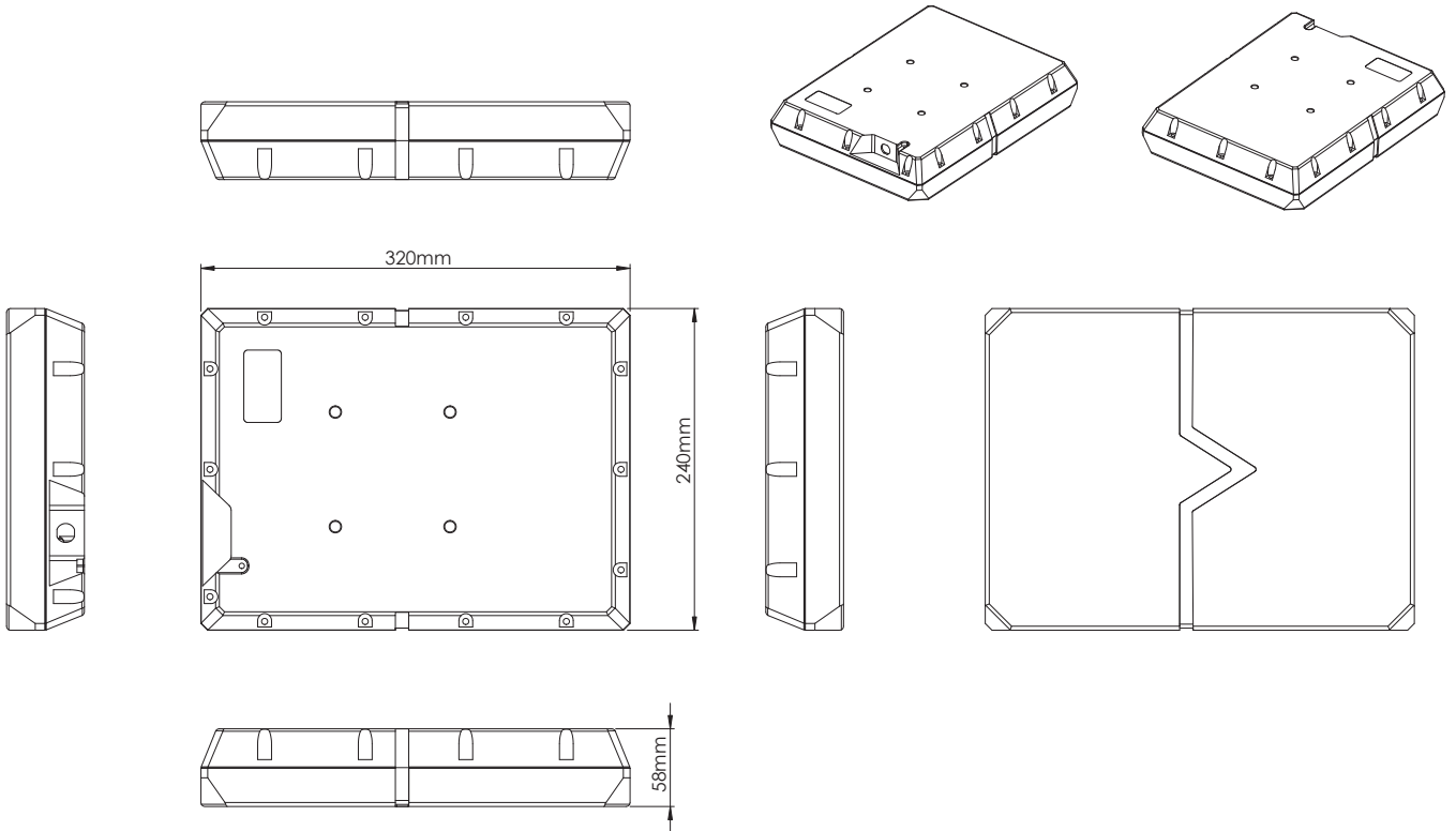
Figure 2: SR-1000 & Scepter-C radar sensor outline drawing
