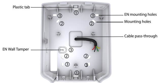
Figure 3: K32LCD+ Backplate
