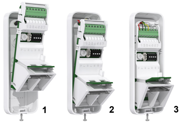
Figure 5 – Attaching the Main Unit
