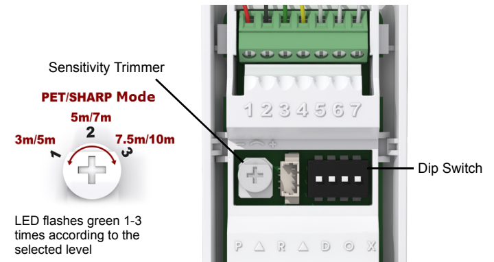
Figure 6 – Detector Settings
