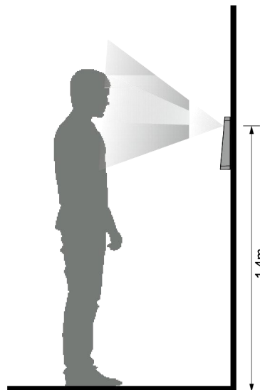
Figure 2-5 Installation height
