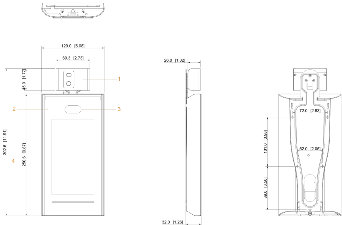
Figure 1-1 Dimensions and components of model X with a temperature monitoring unit (mm [inch])
