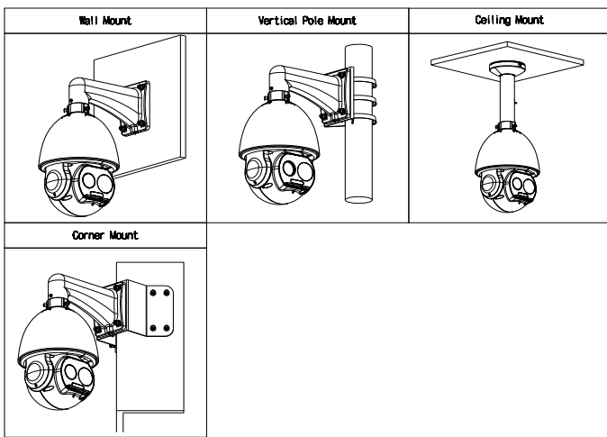
PFB303W + PFA120 + PFA151 Corner Mount Bracket
