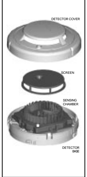
Figure 3: SD-851E Optical Smoke Detector
