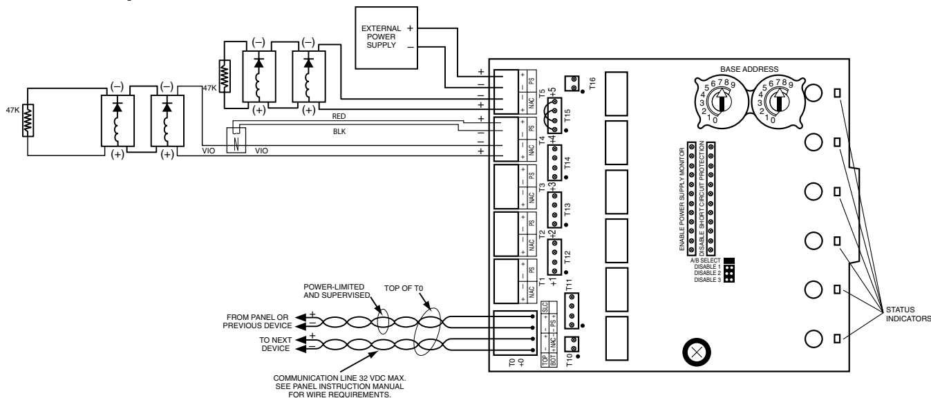
Figure 3: Style Y Monitored Output Circuit configuration with a single supply shared by 2 Monitored Output Circuits.
