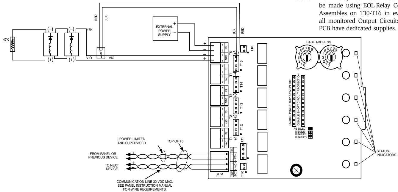
Figure 2: Example of Class B, Style Y Monitored Output Circuit configuration with a single supply dedicated to a single Monitored Output Circuit.
