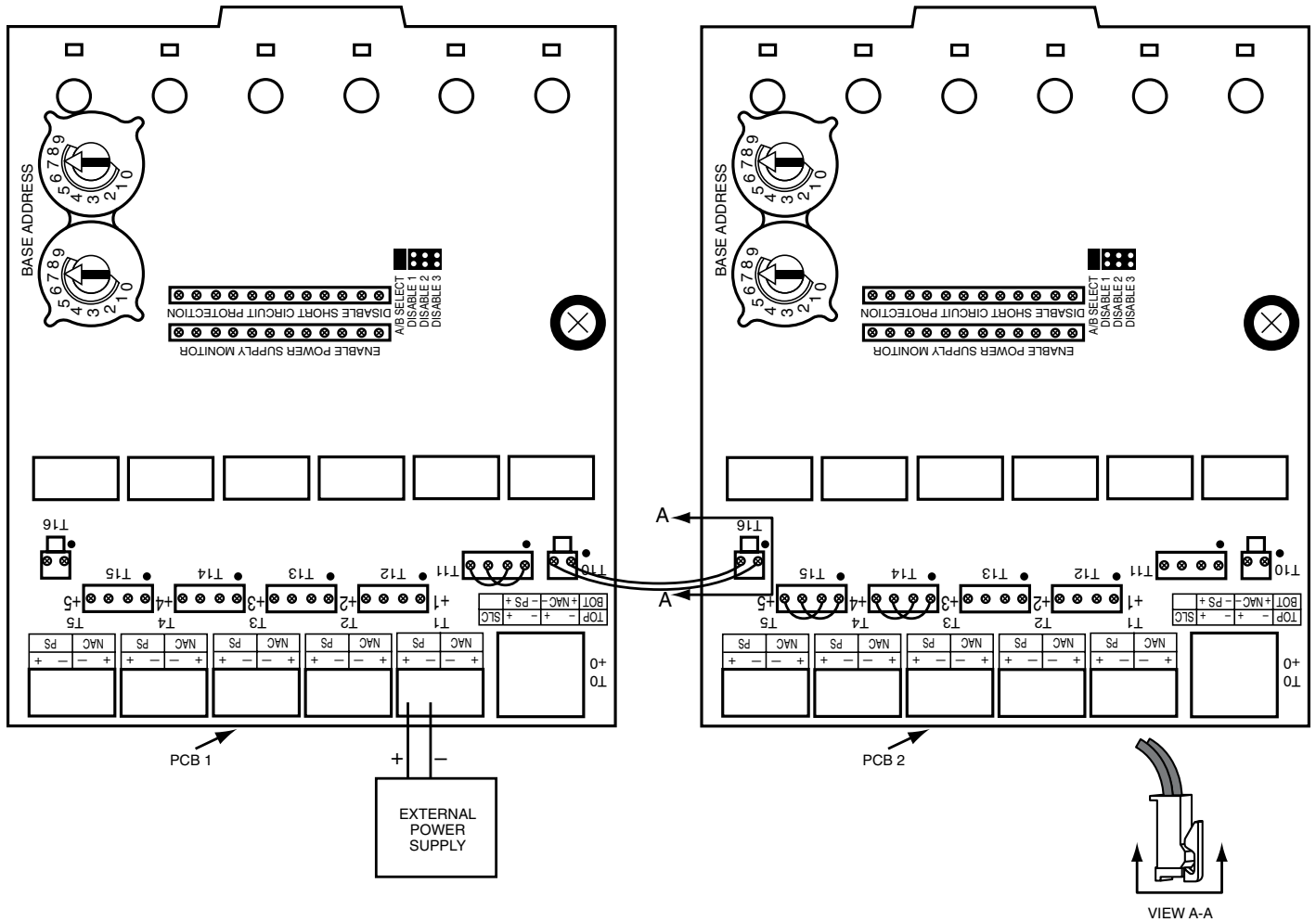
Figure 4: Example of multiple boards sharing same external supply. Supply is shared by Monitored Output Circuits +0 and +1 (on PCB 1) as well as +3, +4, and +5 (on PCB 2). Refer to figure 3 for typical Monitored Output Circuit wiring. Make certain lip on long power supply jumper engages retaining tab on T10 or T16 as shown in View A-A.
