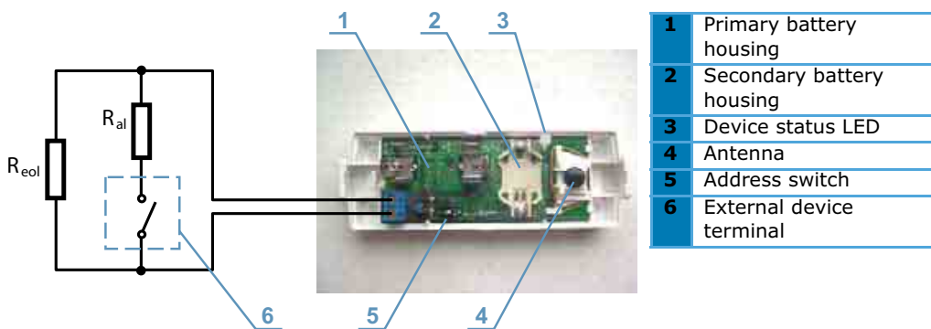
Figure 7 - Terminals
