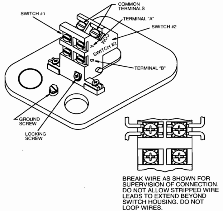
Figure 3. Switch terminals:
